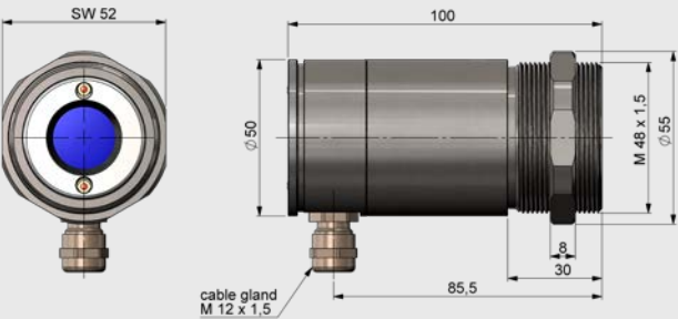
Sensing head
